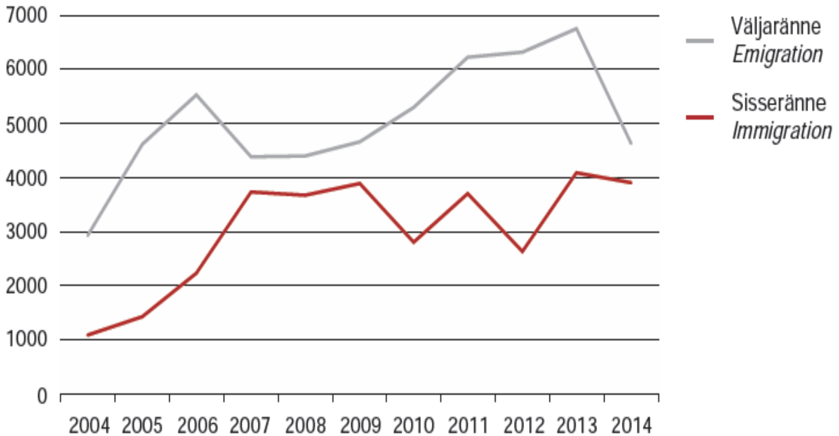
Figure 3. External migration, 2004–2014
